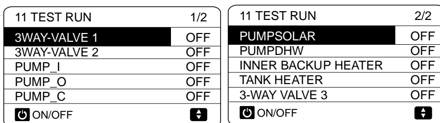
Figure 3-8.34: POINT CHECK menu
