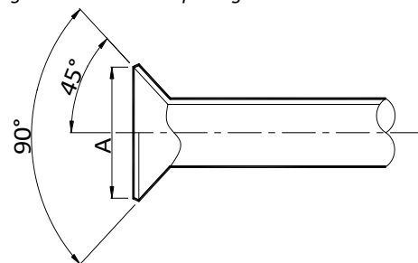
Figure 3-3.3: Flared opening
