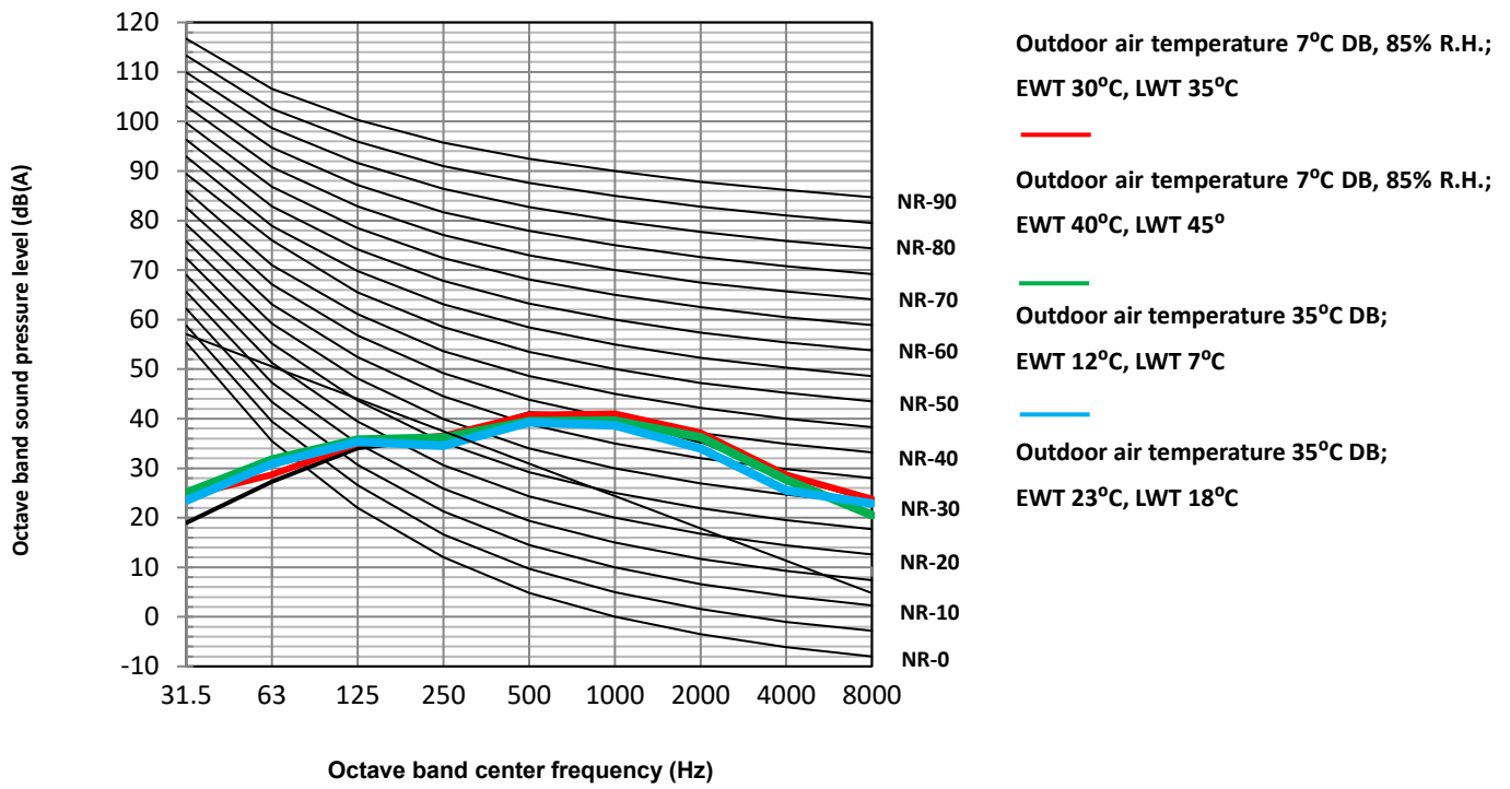
Figure 2-9.2: HOP4WODU octave band levels
