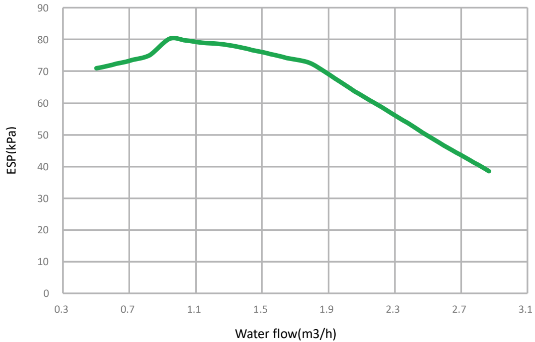
Figure 2-8.2: HOP160WIDU3 hydronic performance
