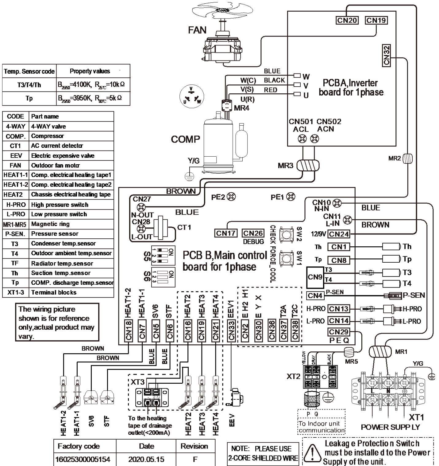
Figure 2-5.1: HOP4(6, 8, 10)WODU wiring diagram
