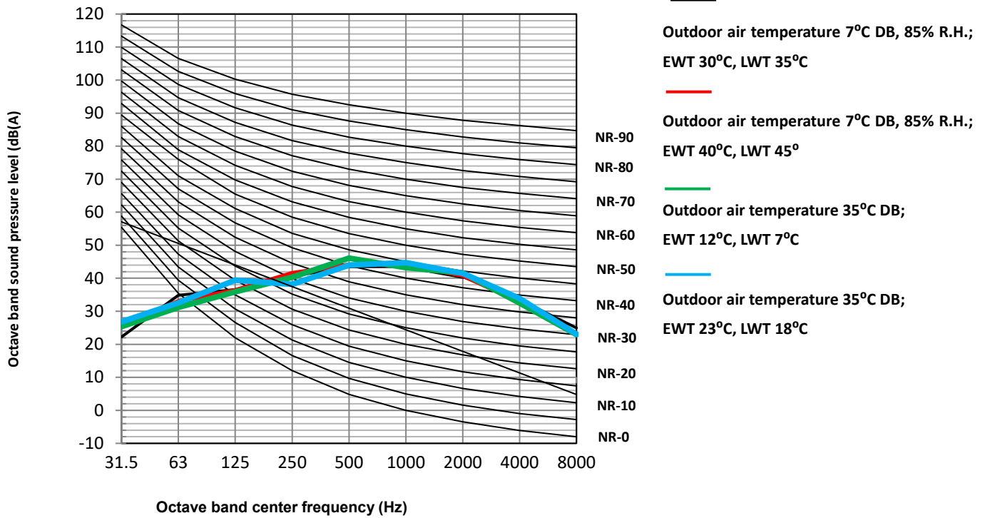
Figure 2-9.4: HOP8WODU octave band levels
