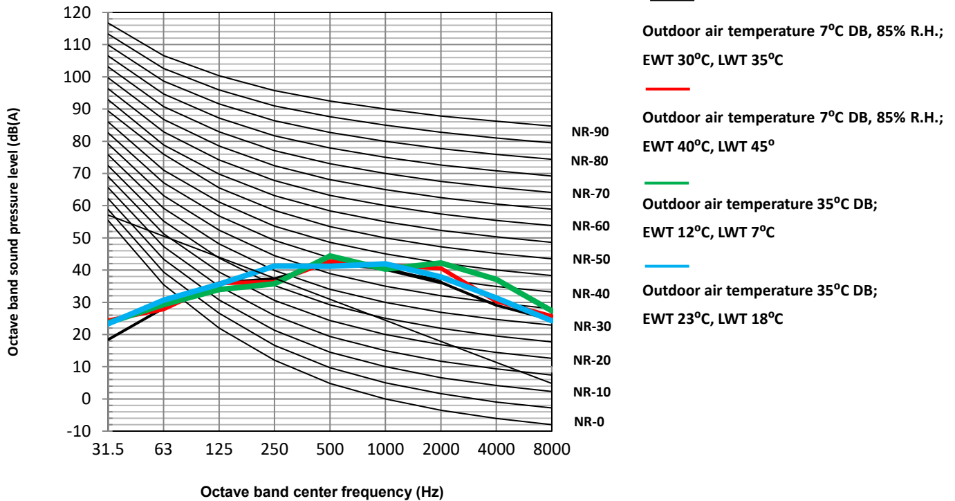
Figure 2-9.3: HOP6WODU octave band levels
