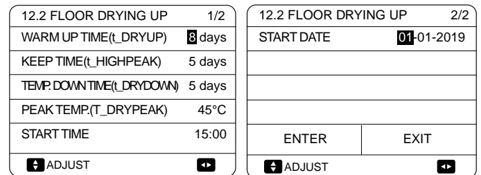
Figure 3-8.44: FLOOR DRYING UP menu
