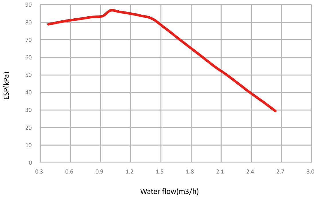
Figure 2-8.1: HOP60(100)WIDU(3) hydronic performance
