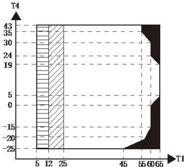
Figure 2-7.3: Domestic hot water operating limits 1
