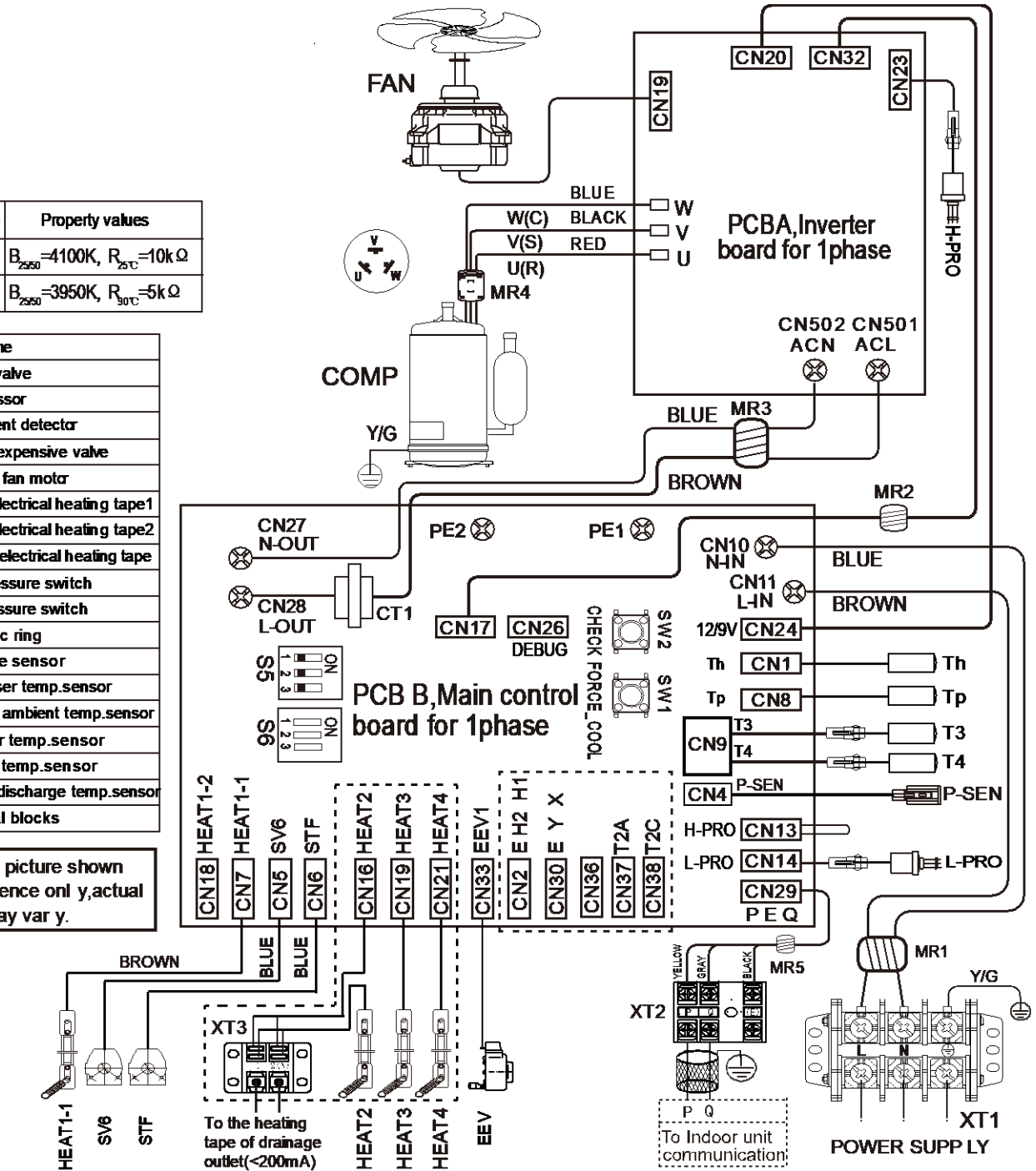
Figure 2-5.1: HOP12(14,16)WODU wiring diagram
