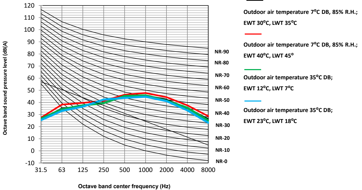
Figure 2-9.5: HOP10WODU octave band levels
