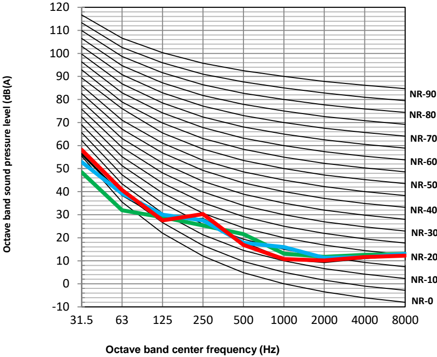
HOP8WODU + HBT-A100/190CD30GN8-B octave band levels
