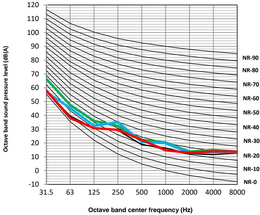
HOP14WODU(3) + HOP160/240IDU (9kW) octave band levels
