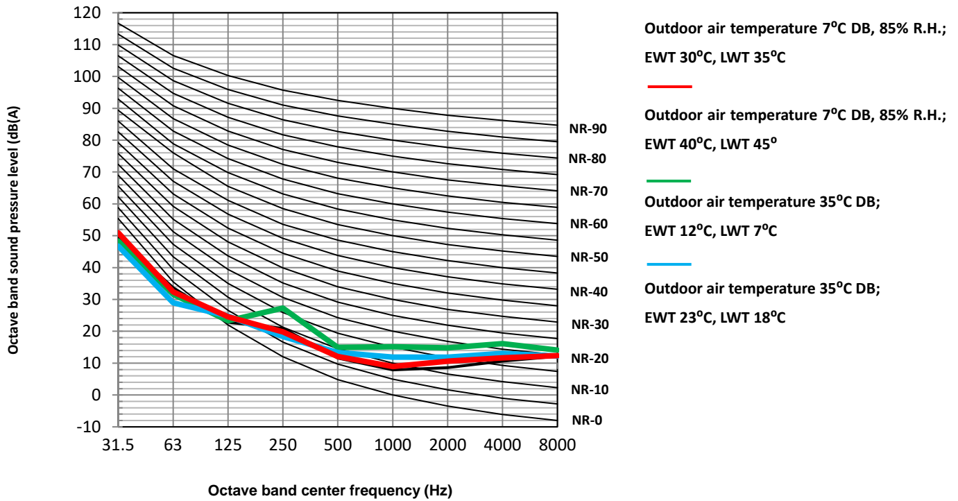
HOP4WODU + HBT-A100/190CD30GN8-B octave band levels
