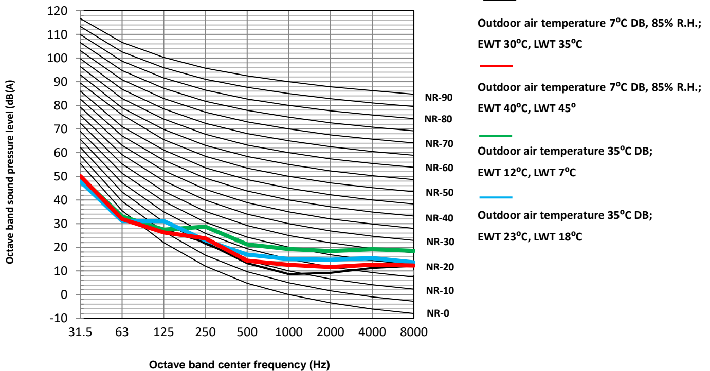
HOP6WODU + HOP100/190IDU(3) (3/9kW) octave band levels
