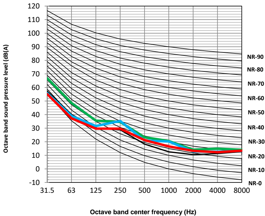
HOP16WODU(3) + HOP160/240IDU (9kW) octave band levels
